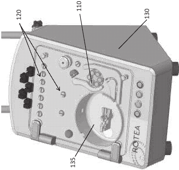
Reusable subsystem 1200
