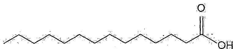
Myristic acid
