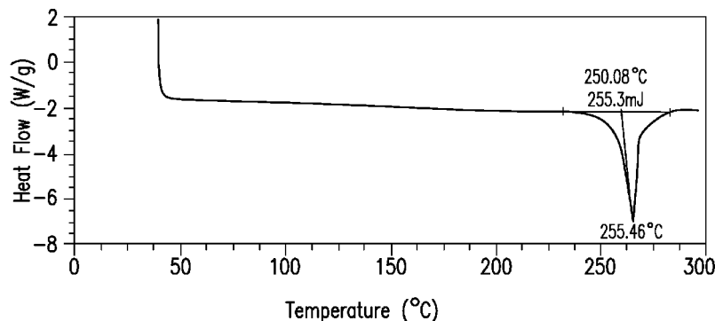
DSC OF (S)-3-4-((4-(MORPHOLINOMETHYL)BENZYL)OXY)-1-OXISOINDOLIN-2-YL)PIPERIDINE-2,6-DIONE HYDROCHLORIDE
