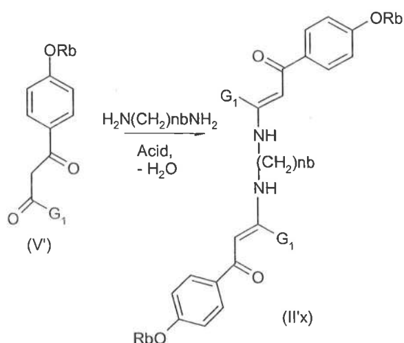
Scheme 4b
