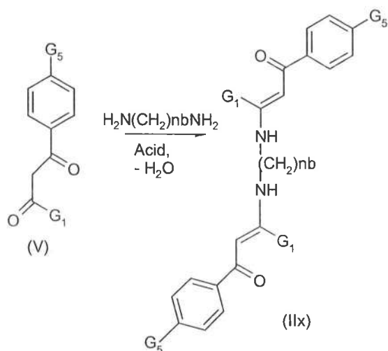
Scheme 4a
