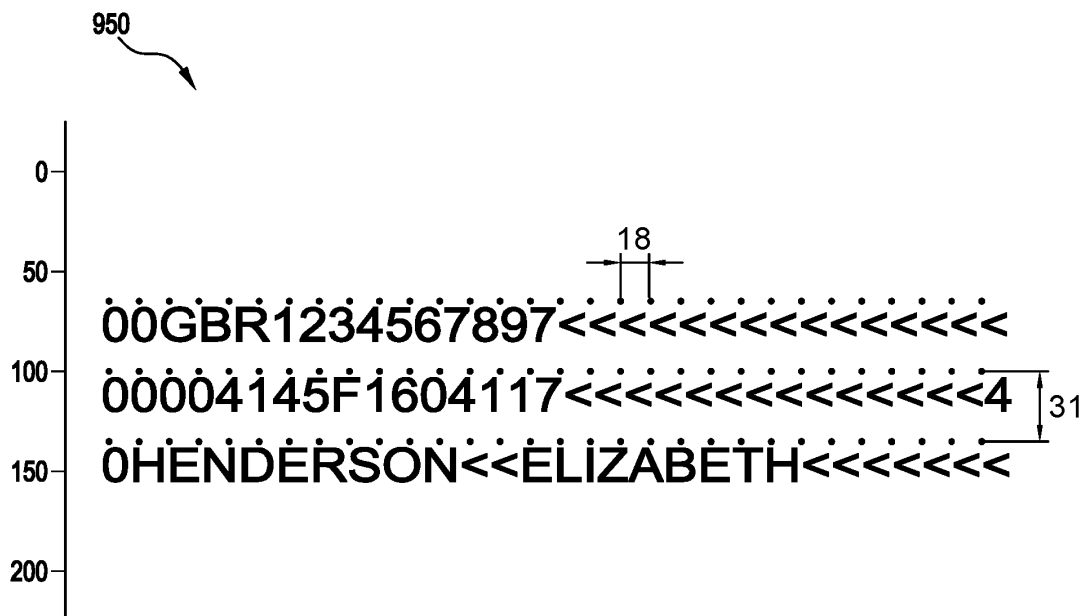
Heuristic Filtering for TD1 for OCRB font
