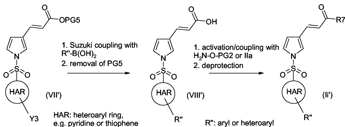
Reaction scheme 5:
