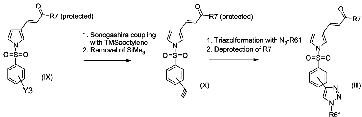
Reaction scheme 6:
