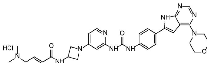
Compound 15
