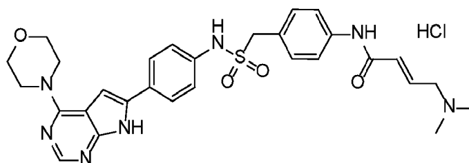
Compound 9
