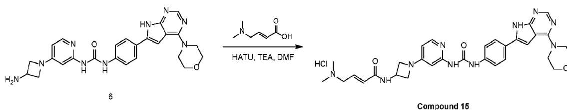
Compound 15
