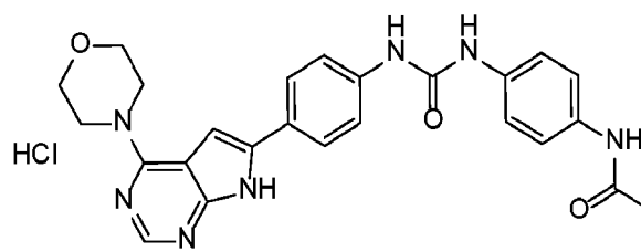
Compound 11
