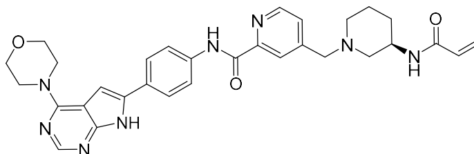
Compound 10
