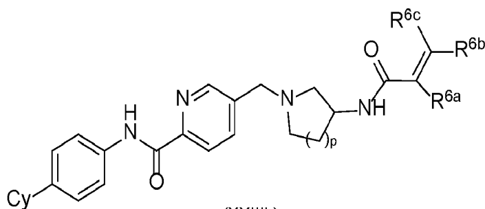
(XXIIIb)
