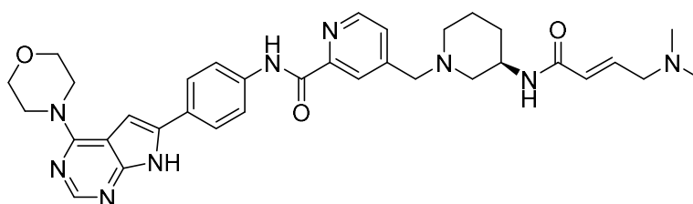
Compound 13
