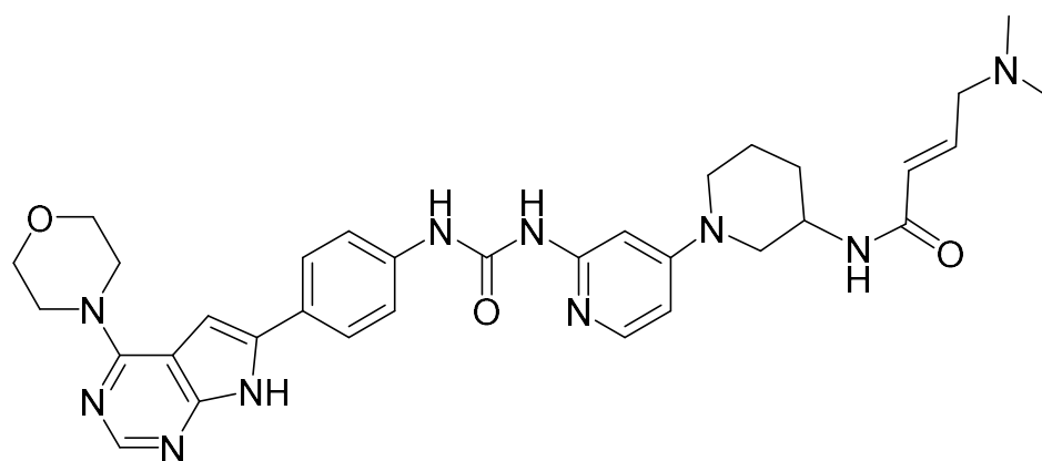
(XIIIc);
