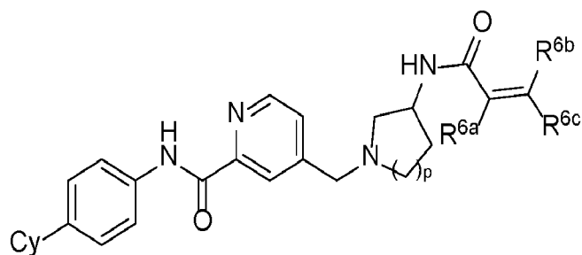
(XXIIIa)
