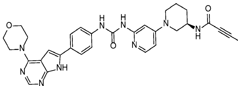
Compound 6
