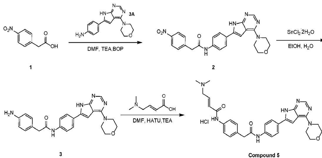
Compound 5
