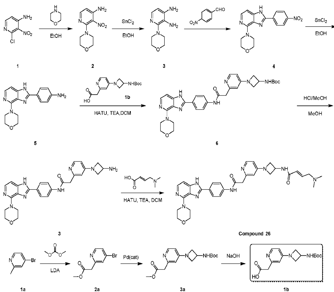
Compound 26
