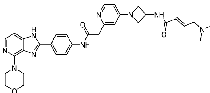
Compound 26
