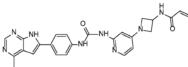
Compound 25
