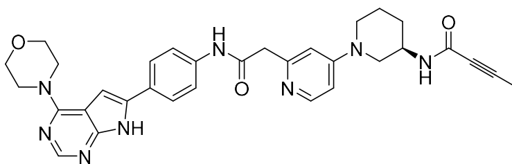
Compound 3
