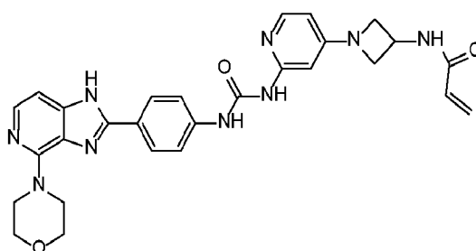
Compound 23
