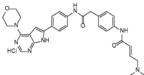
Compound 5
