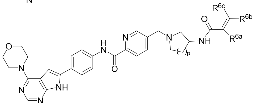
(XXVb),
