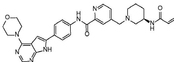
Compound 10
