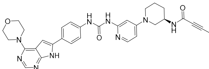
Compound 6
