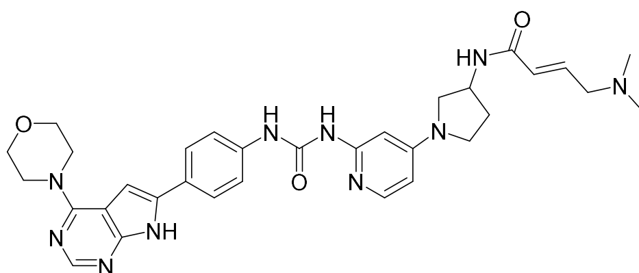
(XIIIb);
