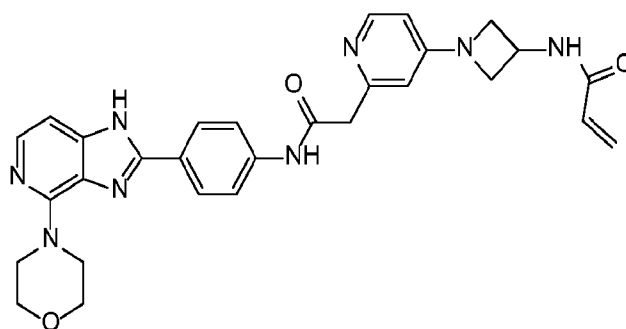
Compound 24
