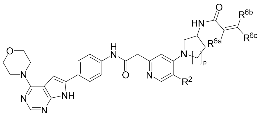
(VIb);
