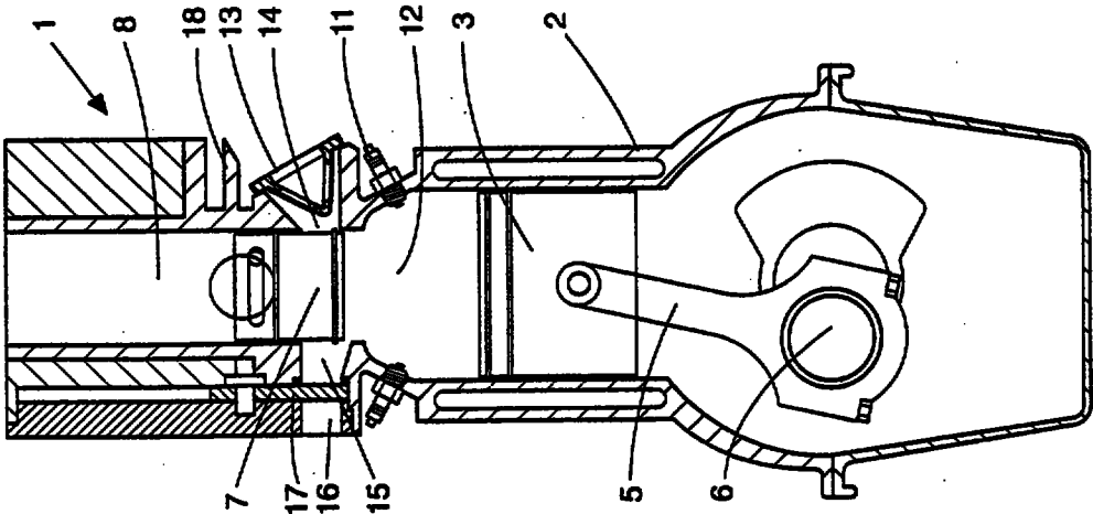
FIGURE 8 630°
