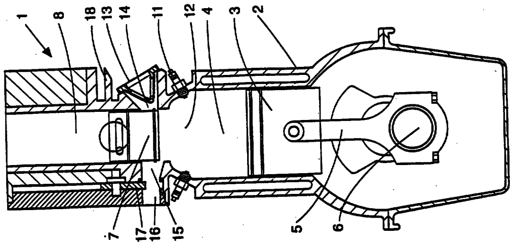
FIGURE 3 BDC 180°
