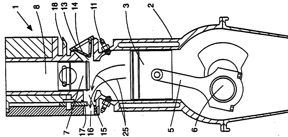
FIGURE 4 TDC 270°
