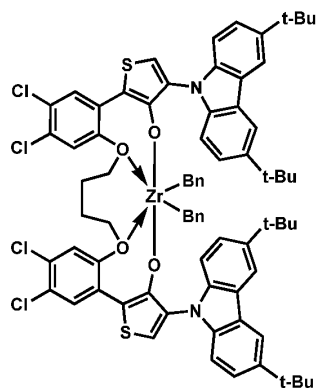
Procatalyst 47
