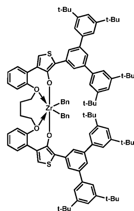
Procatalyst 9
