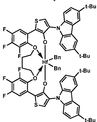
Procatalyst 40
