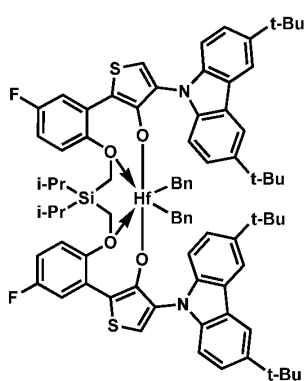
Procatalyst 28
