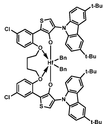
Procatalyst 42
