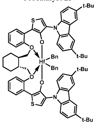
Procatalyst 26
