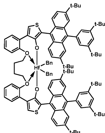
Procatalyst 12
