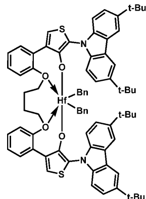
Procatalyst 6
