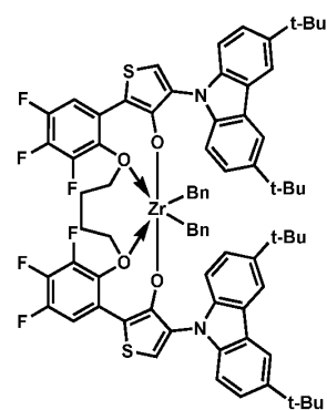
Procatalyst 39
