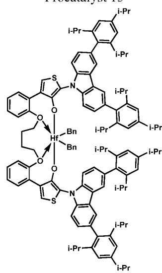
Procatalyst 18
