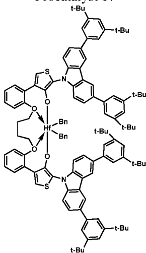
Procatalyst 20
