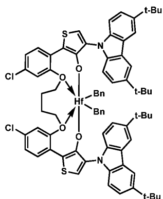
Procatalyst 44
