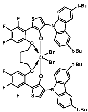
Procatalyst 37
