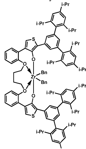
Procatalyst 15
