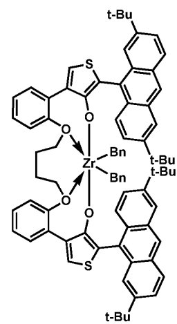
Procatalyst 3
