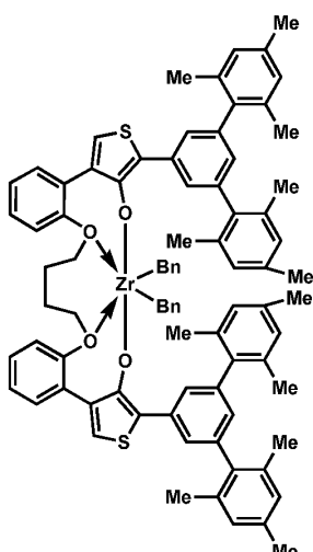
Procatalyst 13
