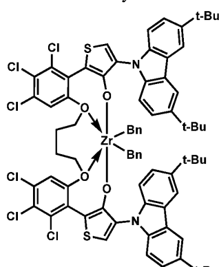
Procatalyst 49
