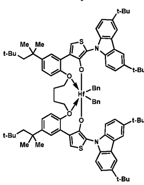
Procatalyst 22
