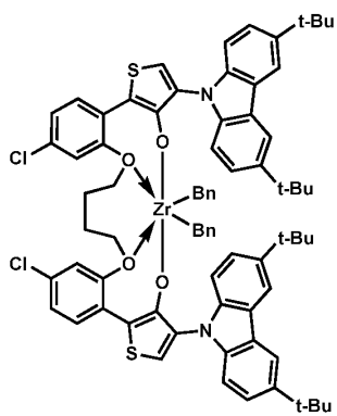
Procatalyst 43
