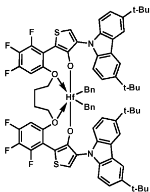
Procatalyst 38
