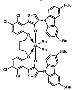
Procatalyst 45
