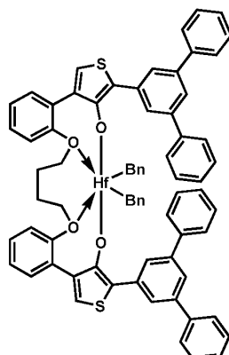
Procatalyst 8
