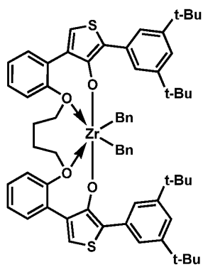
Procatalyst 1
