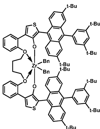
Procatalyst 11
