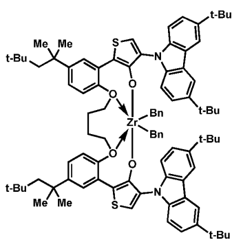
Procatalyst 31
