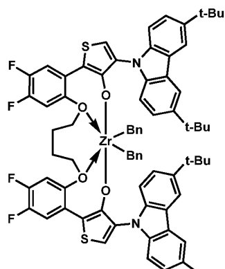
Procatalyst 35
