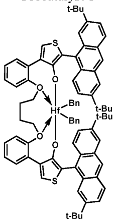
Procatalyst 4
