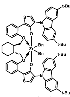
Procatalyst 25
