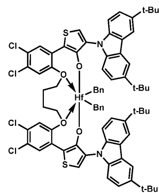
Procatalyst 48
