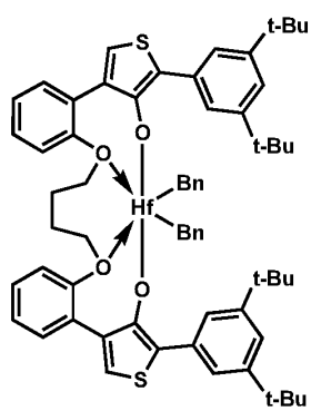
Procatalyst 2
