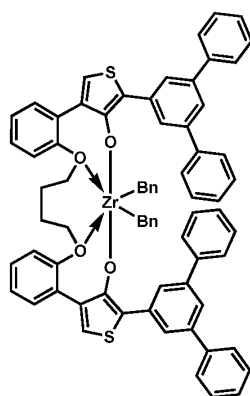
Procatalyst 7
