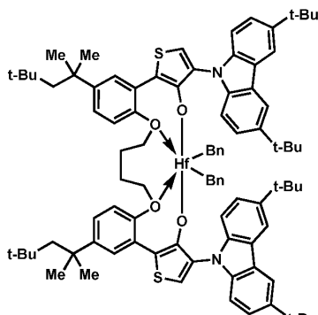
Procatalyst 32
