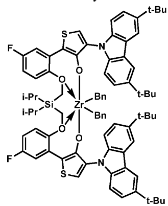
Procatalyst 27
