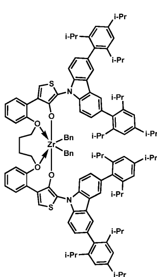
Procatalyst 14
