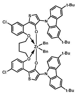
Procatalyst 41
