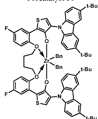
Procatalyst 33
