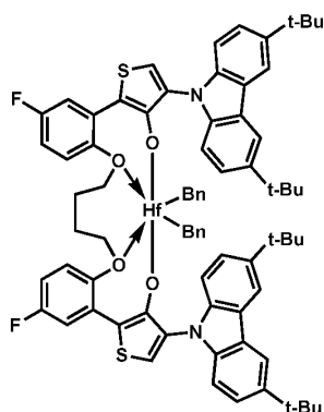
Procatalyst 34
