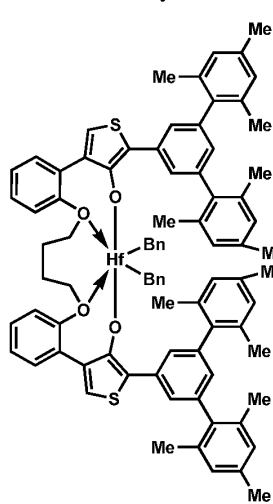
Procatalyst 14
