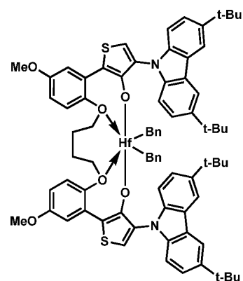
Procatalyst 30
