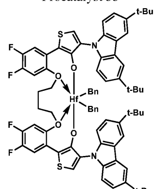
Procatalyst 36
