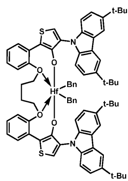
Procatalyst 24
