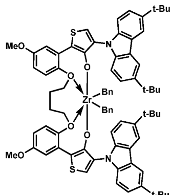
Procatalyst 29
