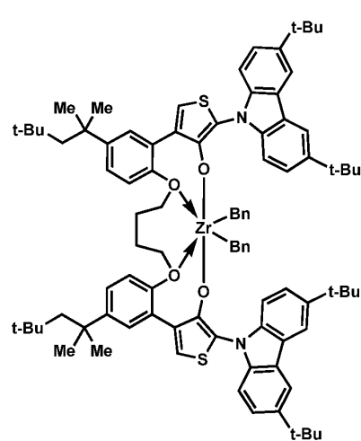
Procatalyst 21
