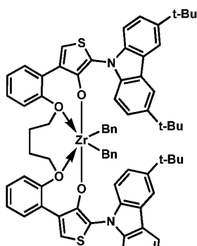
Procatalyst 5
