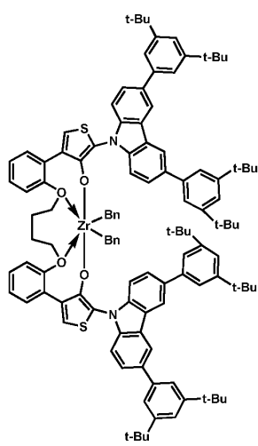
Procatalyst 19
