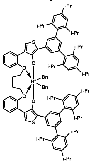
Procatalyst 16
