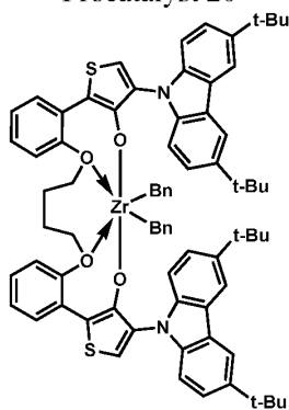
Procatalyst 23
