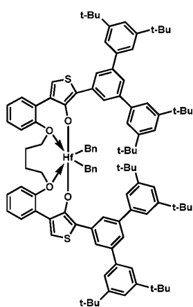
Procatalyst 10
