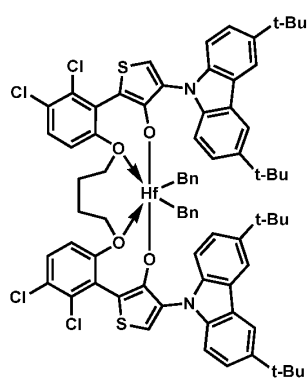
Procatalyst 46
