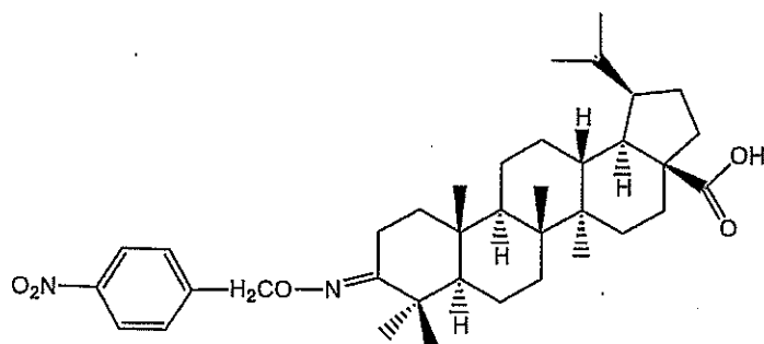
MJ-1098 (II), As Disclosed In US 6,403,816
