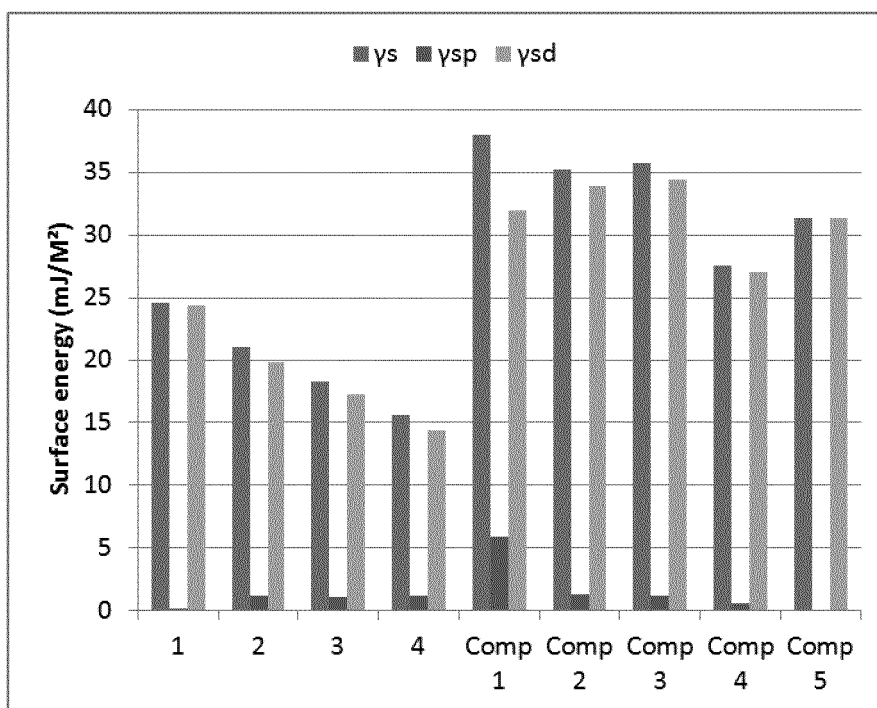
Figure 3 : Surface energies determined by the Owens-Wendt method
