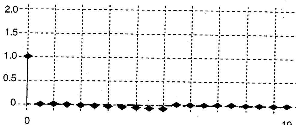
AUTOCORRELATION ANALYSIS
