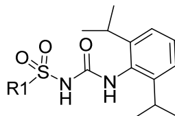
formula (Ib)
