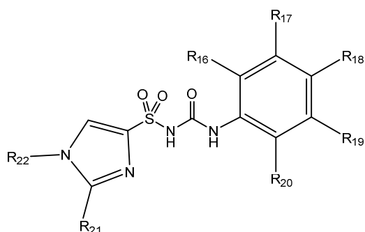
Formula (IVa)
