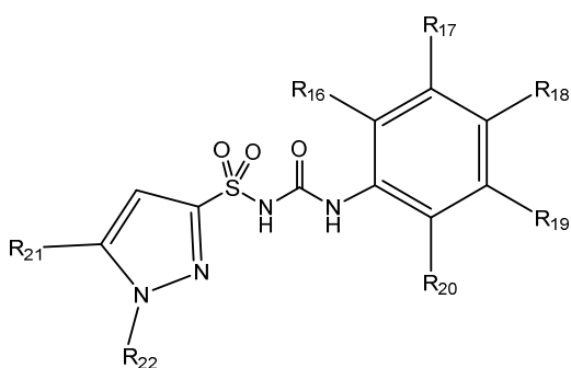
Formula (IIIa)
