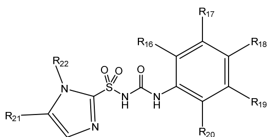
Formula (IVb)
