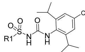
formula (Ic)
