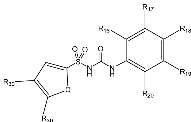
Formula (VII)
