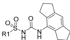
formula (Ia)
