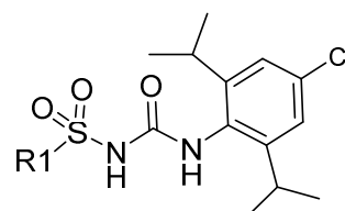
formula (Ic)
