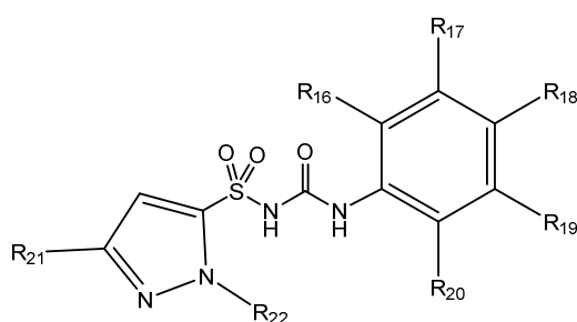
Formula (IIIb)
