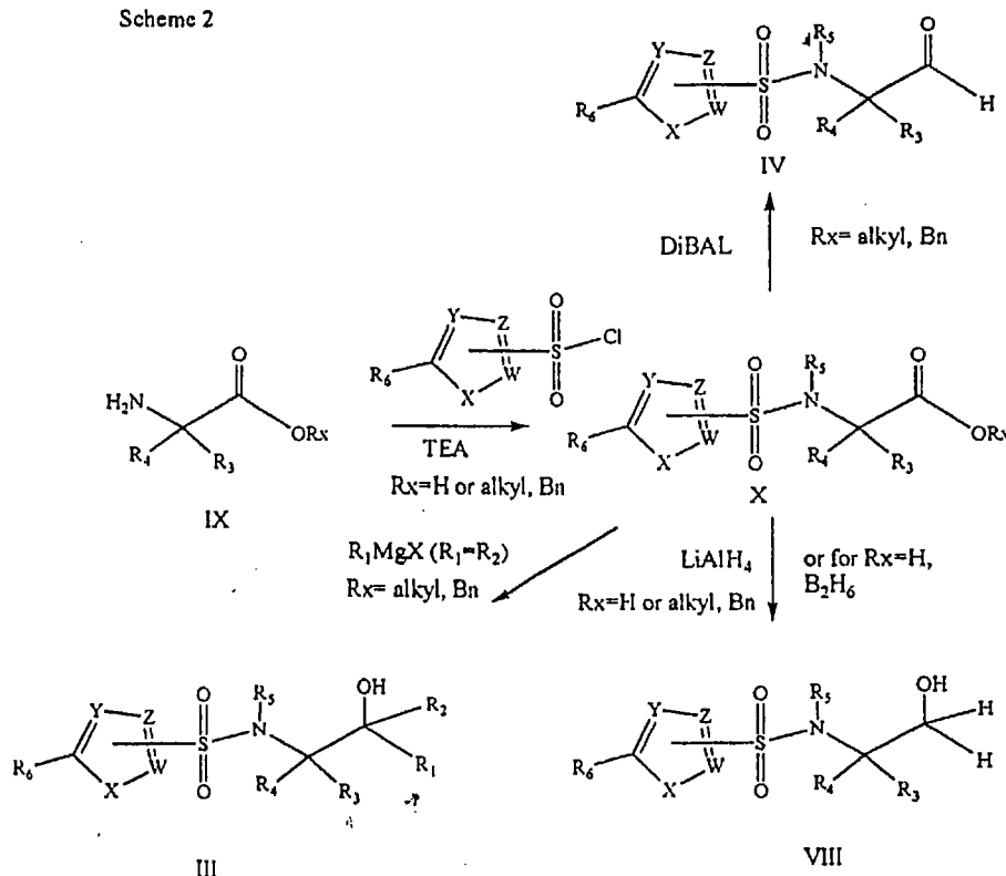
Scheme 2
