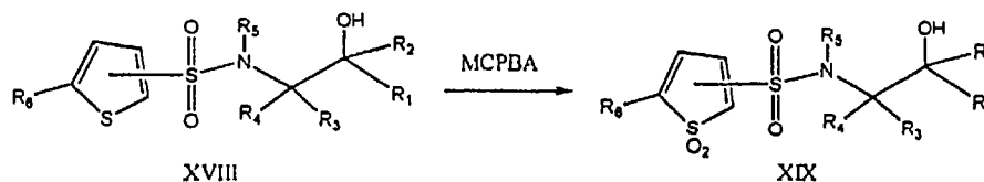
Scheme 6
