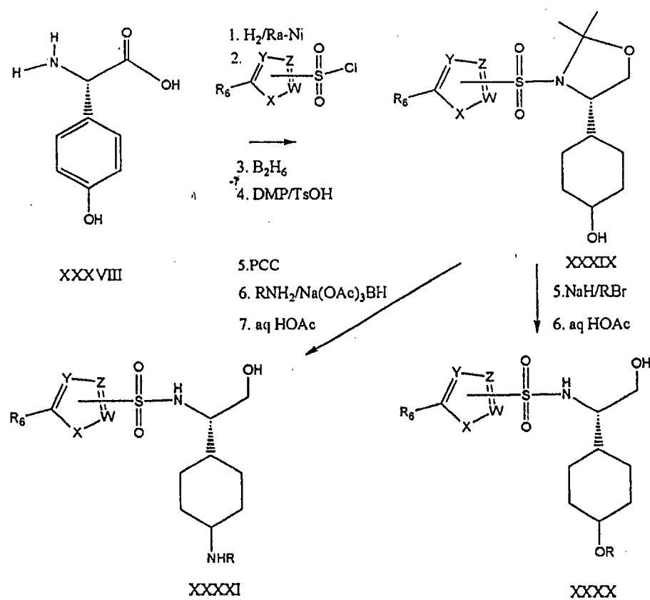
Scheme 12
