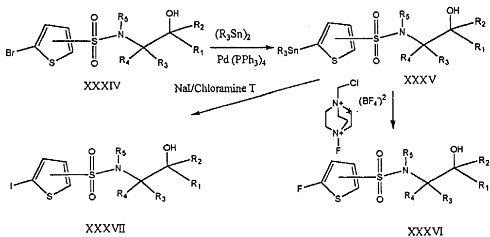
Scheme 12
