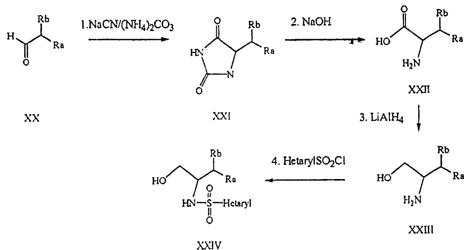
Scheme 7
