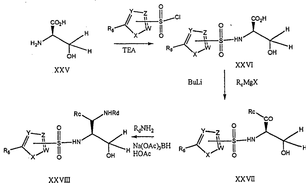
Scheme 8
