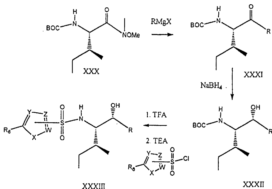
Scheme 10
