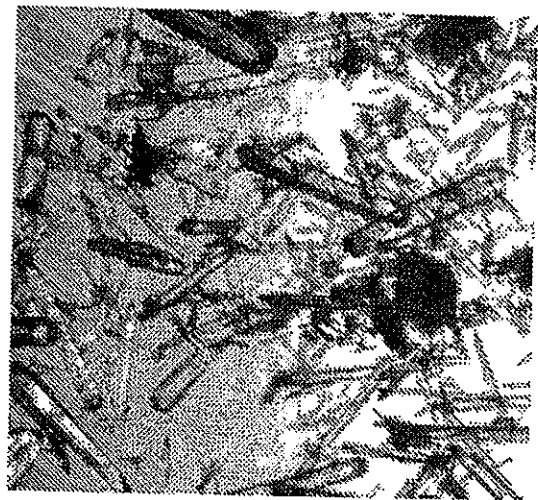
Crystal Form 3
