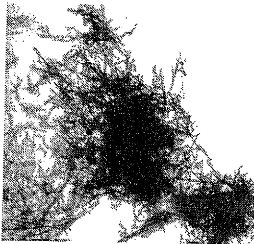
Crystal Form 1
