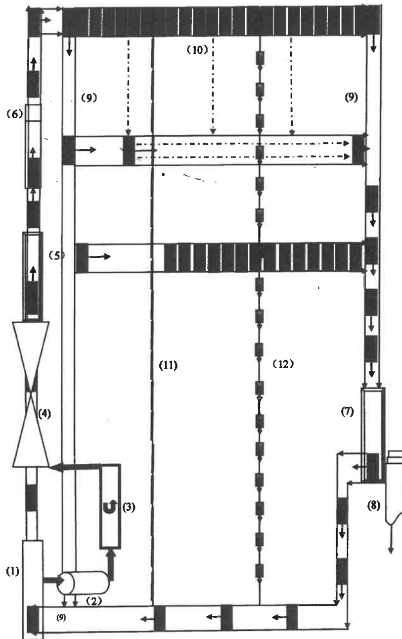
FIG.2: Full-automatic Parallel-moving Tray Type Organic plants Growing System
