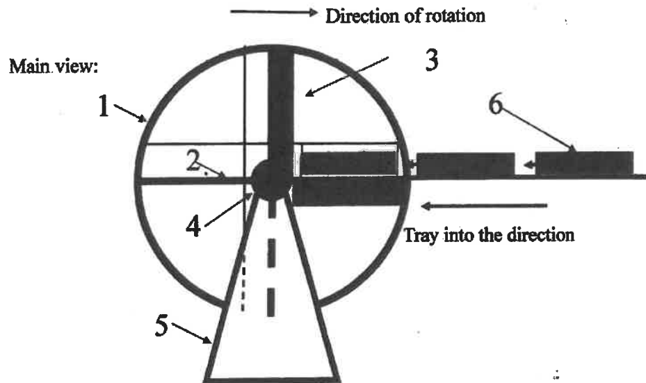
FIG.3 An after-grown tray previously grown material turning and dumping system
