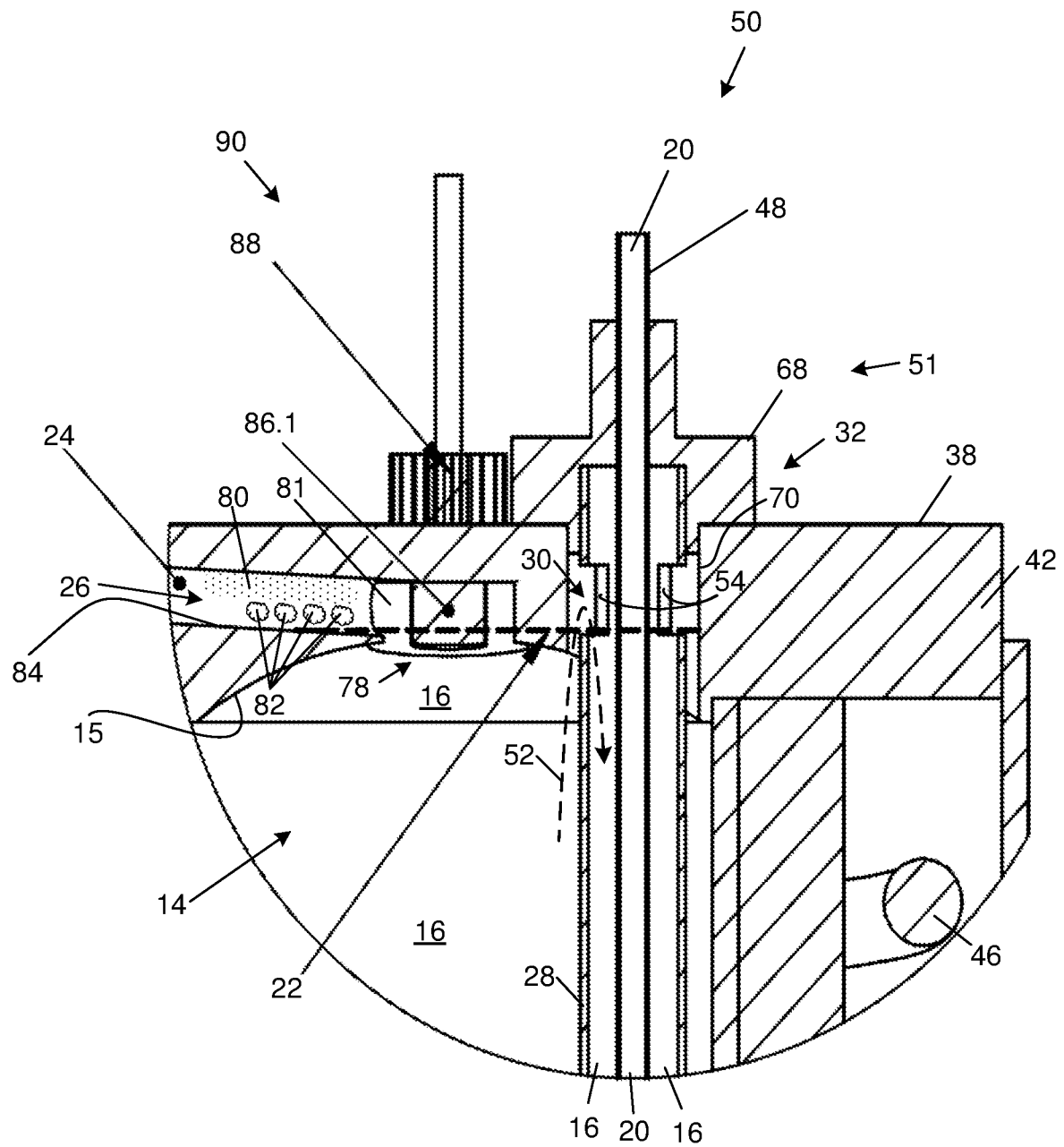
DETAIL H
