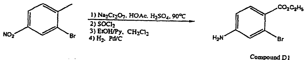
Reaction Scheme 6
