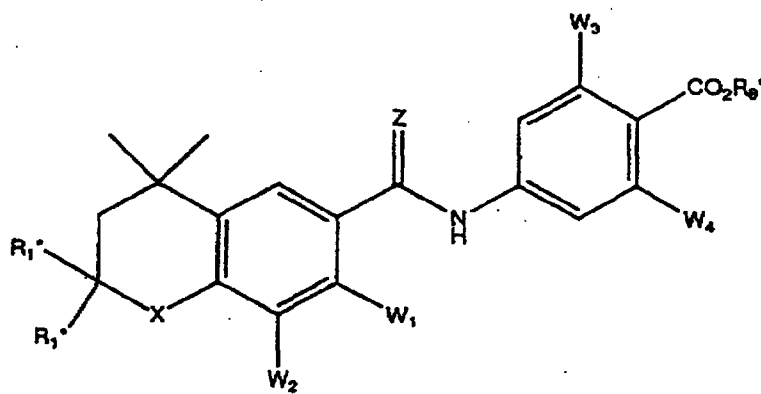
Formula 5
