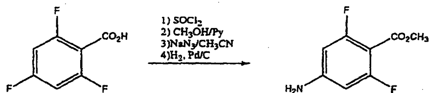
Compound G1
