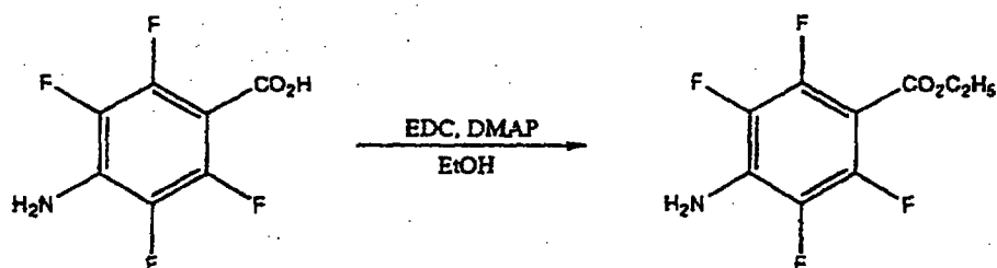
Compound G1
