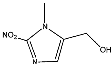
N-1-methyl-2-nitro-5-hydroxymethyl imidazole
