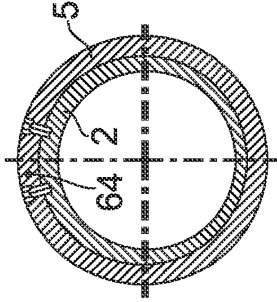
Section 'J-J'
