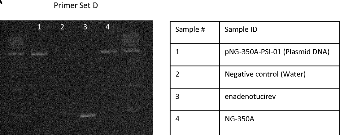
Figure 6 PCR Products
