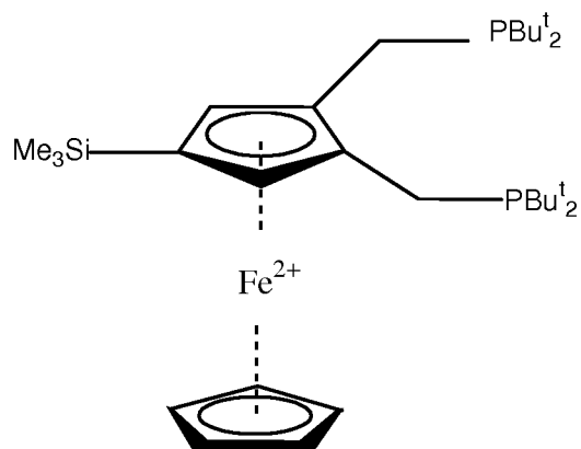
1,2-bis(di-tert-butylphosphinomethyl)-4-trimethylsilyl ferrocene
