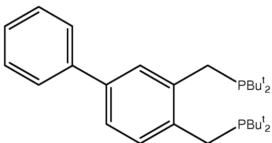
1,2-bis(di-tert-butyl(phosphinomethyl))-4-phenyl benzene
