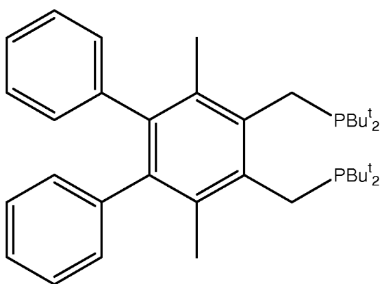
1,2-bis(di-tert-butyl(phosphinomethyl))-3,6-dimethyl-4,5-diphenyl benzene
