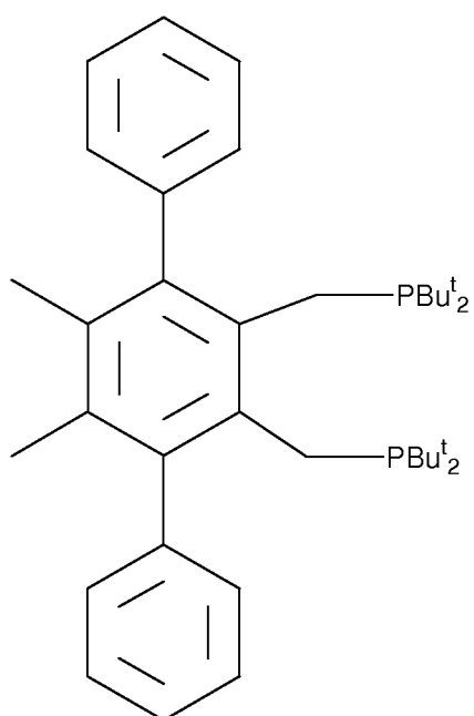
1,2-bis(di-tert-butylphosphinomethyl)-3,6-diphenyl-4,5-dimethylbenzene
