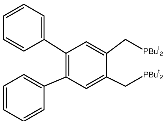
1,2 bis(di-tert-butyl(phosphinomethyl)-4,5-diphenyl benzene
