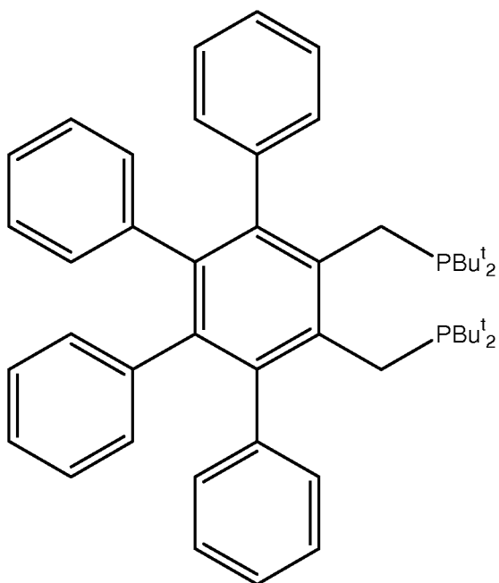
1,2-bis(di-tert-butyl(phosphinomethyl))-3,4,5,6-tetraphenyl benzene
