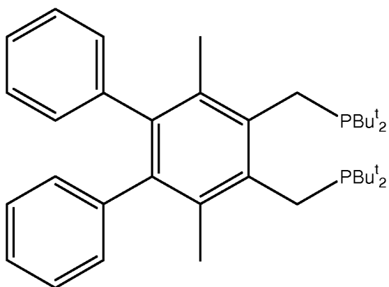
1,2-bis(di-tert-butyl(phosphinomethyl))-3,6-dimethyl-4,5-diphenyl benzene
