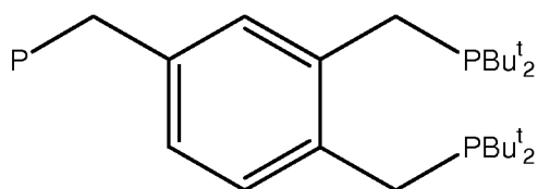
1,2-bis(di- tert -butyl (phosphinomethyl))-4-(phosphinomethyl)benzene
