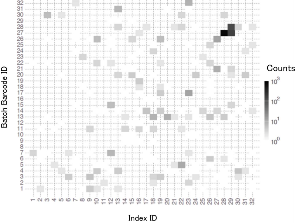
FIG. 16 Misdetermined RNA ID – counts
