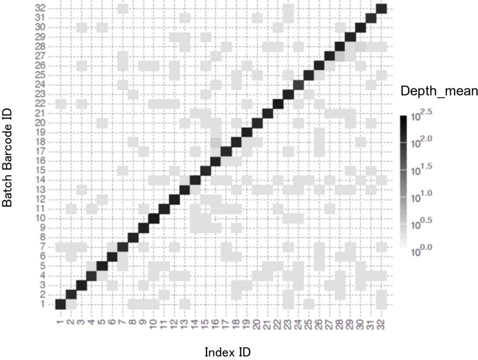
FIG. 15 Structured Batch RNA Barcodes – sequence read depth
