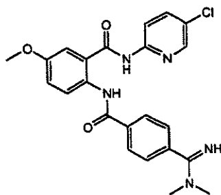
Compound A.
