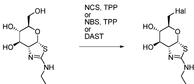
Scheme 1: Reaction sequence for compounds of sub-formula (IA-1)
