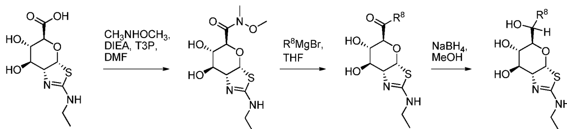
Scheme 4: Reaction sequence for compounds of sub-formula (IC)
