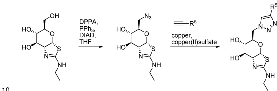
Scheme 2: Reaction sequence for compounds of sub-formula (IA-2)
