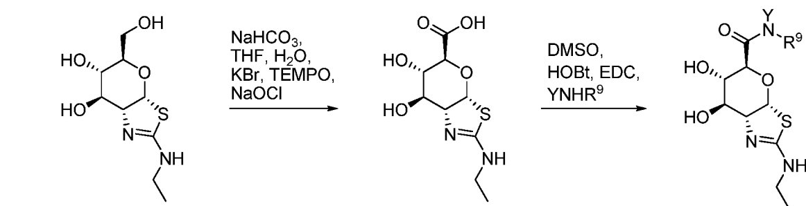
Scheme 3: Reaction sequence for compounds of sub-formula (IB-1)
