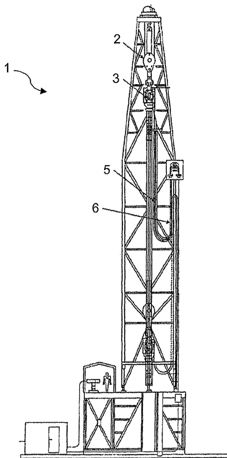
FIG. 4 (PRIOR ART)
