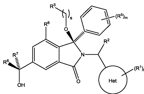
Diastereoisomer 2B
