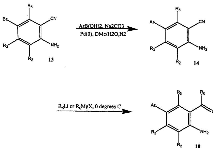
Scheme III
