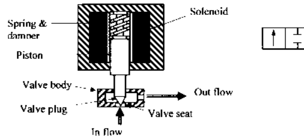
Fig 5. - A schematic of a solenoid operated 2/2 poppet valve and symbol
