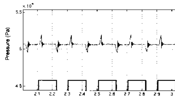
Fig 6. - PWM at a typical ON-OFF operation frequency 5 Hz of a solenoid poppet valve and the corresponding pressure in the system
