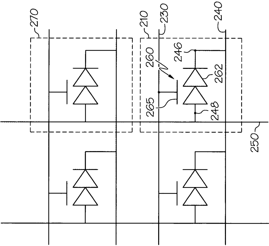
FIG. 2 (PRIOR ART)
