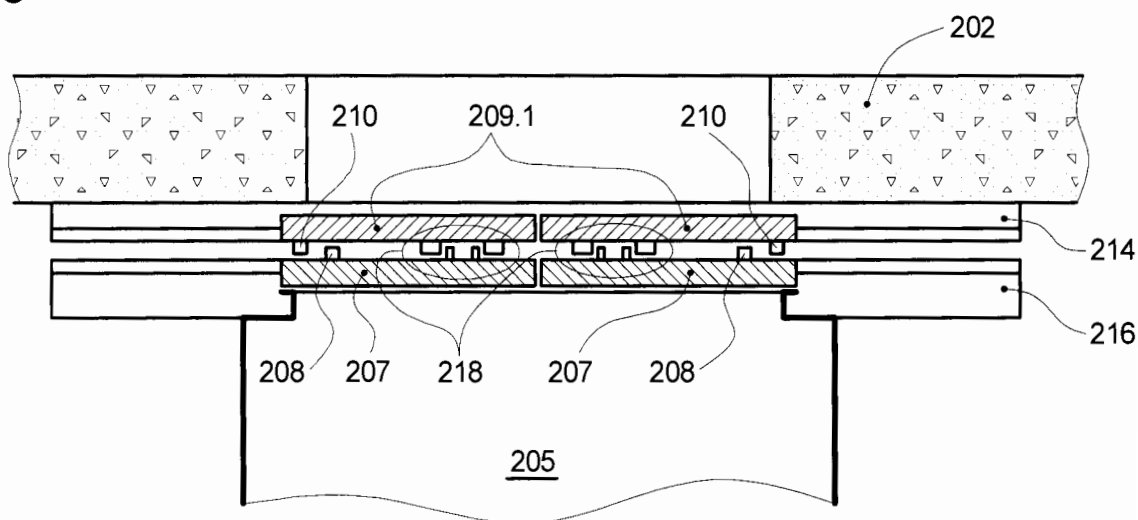
Fig. 3 (Section III-III)
