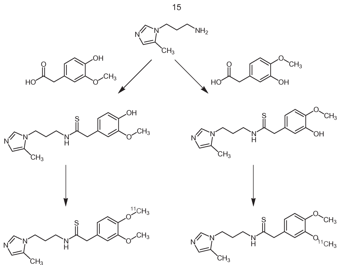
Scheme A
