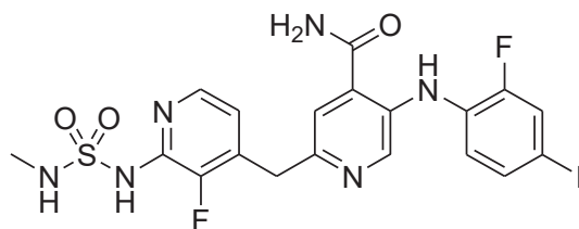
[Chemical Formula 282]
