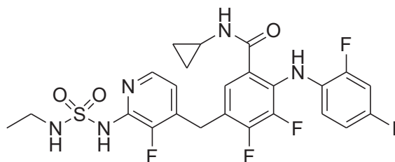
[Chemical Formula 56]
