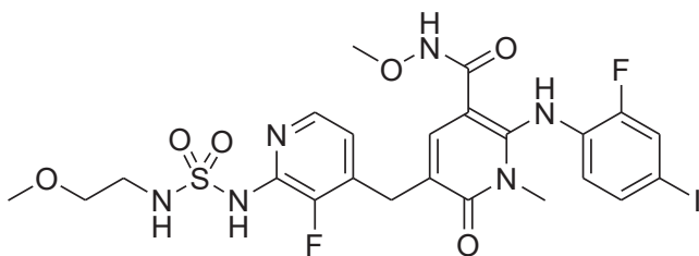
[Chemical Formula 247]
