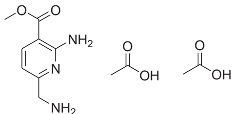
[Chemical Formula 283]
