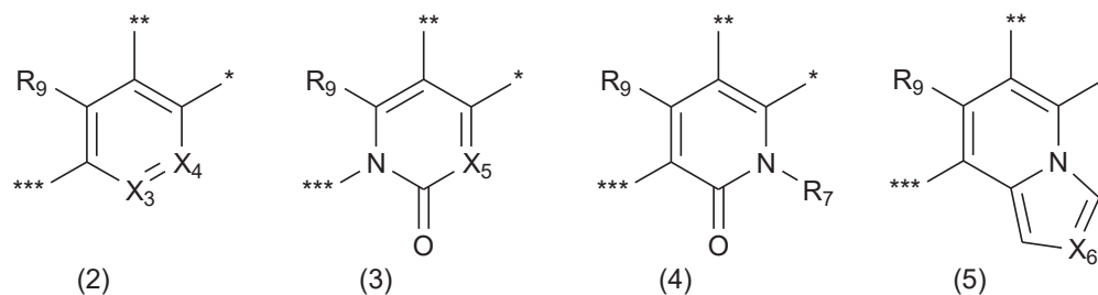
[Chemical Formula 5]
