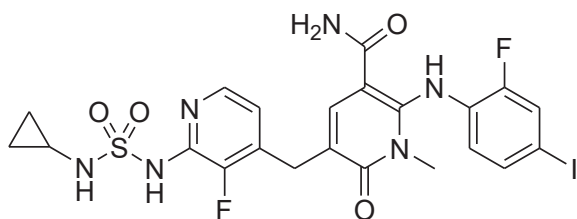
[Chemical Formula 250]
