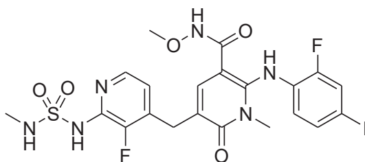
[Chemical Formula 246]
