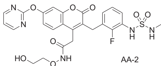
[Chemical Formula 3]
