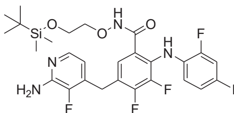
[Chemical Formula 108]
