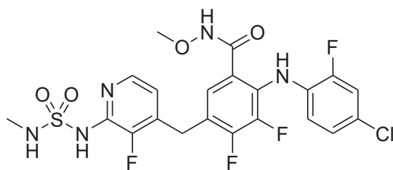
[Chemical Formula 210]
