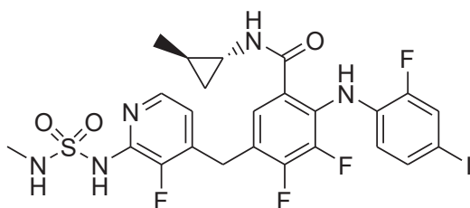
[Chemical Formula 130]
