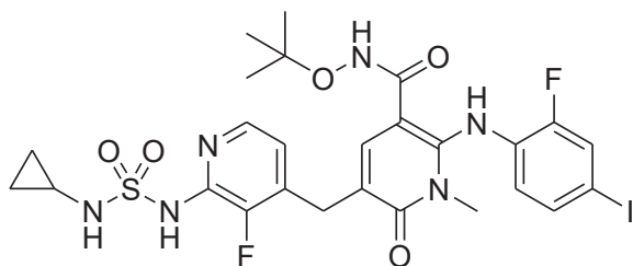
[Chemical Formula 249]
