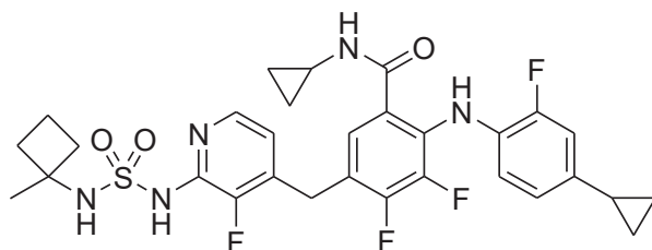
[Chemical Formula 211]
