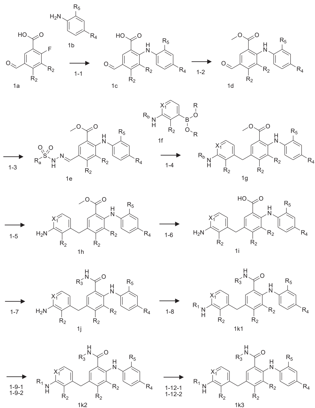
[Chemical Formula 22]
