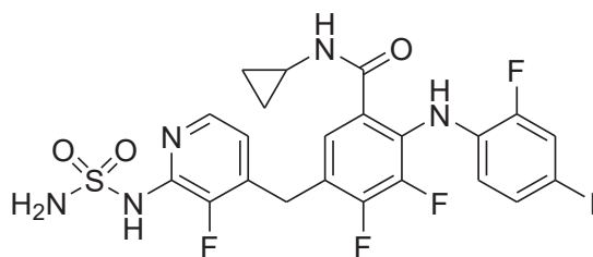
[Chemical Formula 55]
