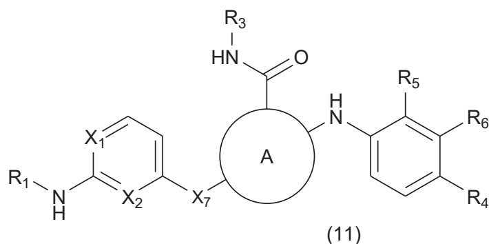
[Chemical Formula 4]
