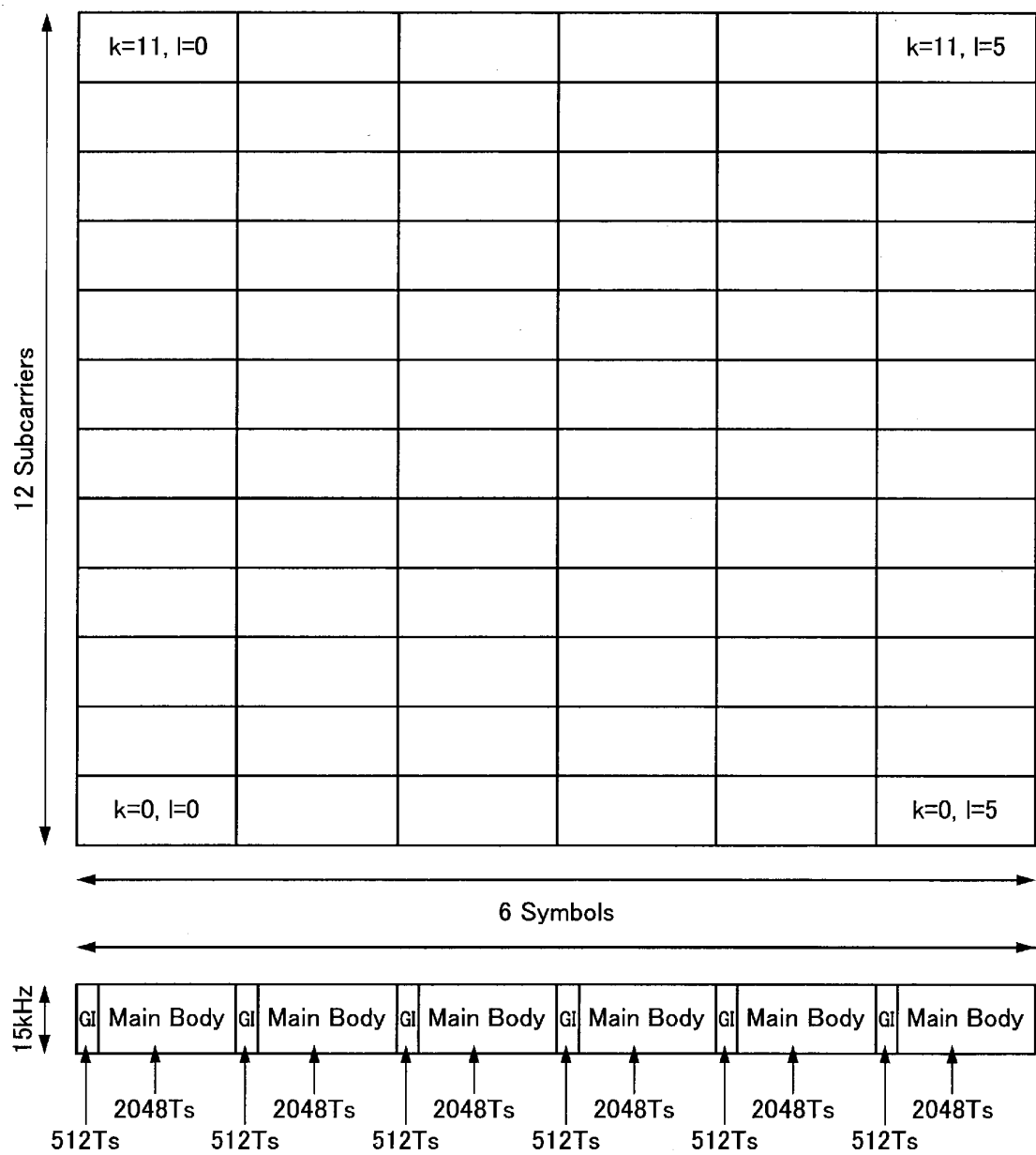
Case 2 : Extended Guard Interval 15kHz Subcarriers
