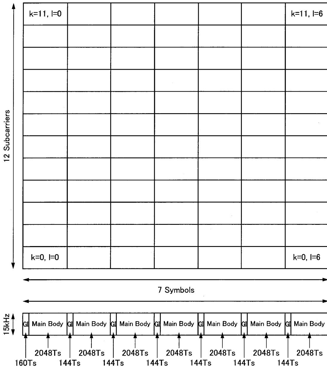
Case 1 : Normal Guard Interval 15kHz Subcarriers
