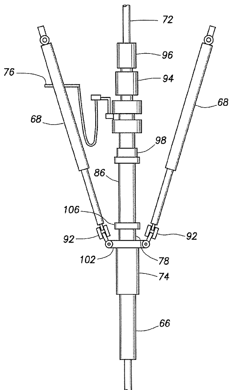
FIG. 4 (PRIOR ART)
