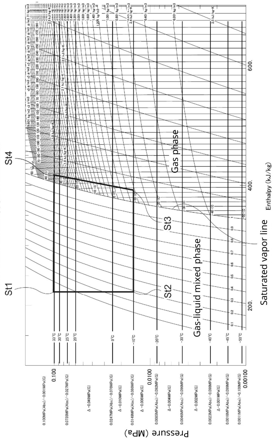
5: Pressure vs. Enthalpy plot: R1336mzz(Z)
