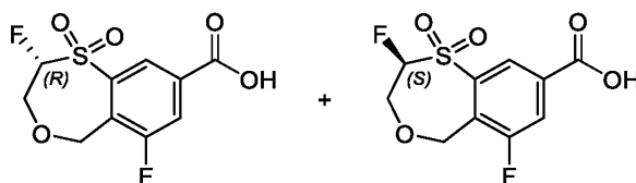
Intermediate 1
