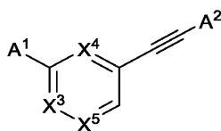
Formula C
