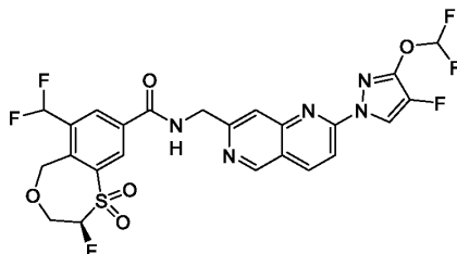
Compound 514
