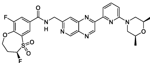
Compound 405
