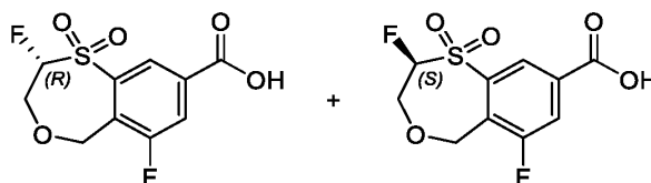
Intermediate 4
