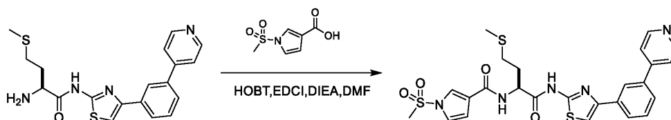
Compound B
