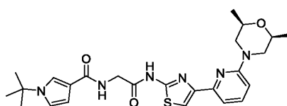
Compound C
