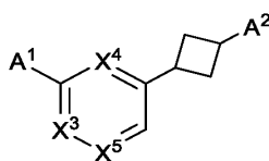
Formula D
