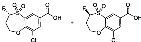
Intermediate 3
