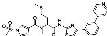
Compound B
