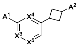
Formula D
