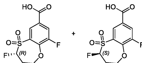
Intermediate 2
