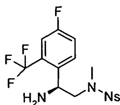
(S)-1-(4-fluoro-2-(trifluoromethyl)phenyl)-N,N'-dimethylethane-1,2-diamine (46)
