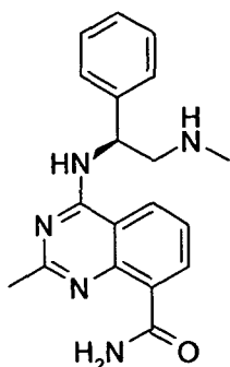
2-Methyl-4-[[[(1S)-2-(methylamino)-1-phenylethyl]amino]quinazoline-8-carboxamide (26)
