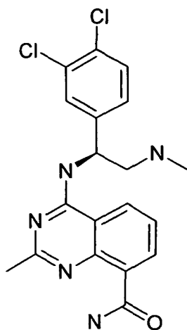
(S)-4-((1-(3,4-dichlorophenyl)-2-(methylamino)ethyl)amino)-2-methylquinazoline-8-carboxamide (61)
