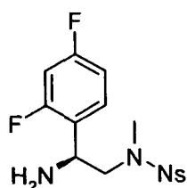
(S)-N-(2-amino-2-(2,4-difluorophenyl)ethyl)-N-methyl-4-nitrobenzenesulfonamide (42)
