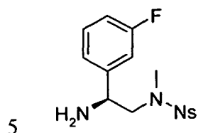
N-[(2S)-2-amino-2-(3-fluorophenyl)ethyl]-N-methyl-4-nitrobenzenesulfonamide (10)
