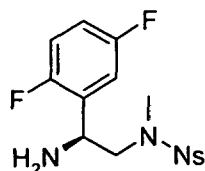
(S)-N-(2-amino-2-(2,5-difluorophenyl)ethyl)-N-methyl-4-nitrobenzenesulfonamide (44)
