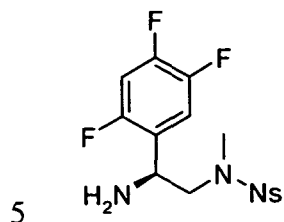
(S)-N-(2-amino-2-(2,4,5-trifluorophenyl)ethyl)-N-methyl-4-nitrobenzenesulfonamide (45)
