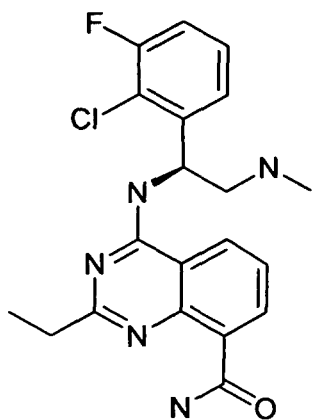
(S)-4-((1-(2-chloro-3-fluorophenyl)-2-(methylamino)ethyl)amino)-2-ethylquinazoline-8-carboxamide (60)
