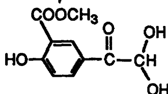
5-Glyoxyloyl-salicylic acid methyl ester hydrate
