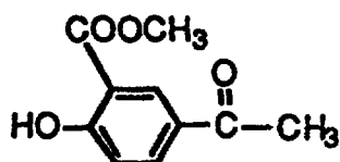
Methyl 5-Acetylsalicylate
