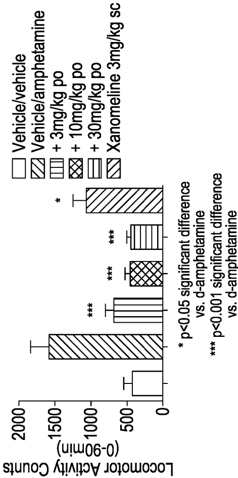
Example 1-33 Isomer 2
