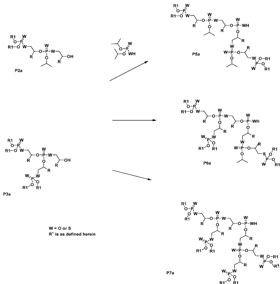
Scheme 4
