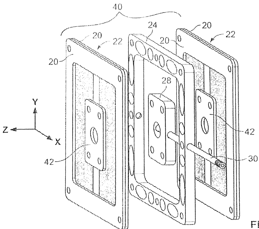
FIG. 3 (Prior Art)
