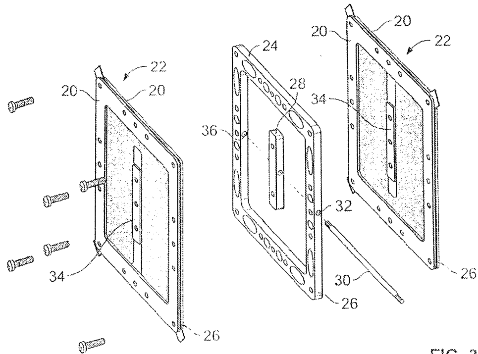
FIG. 3 (Prior Art)
