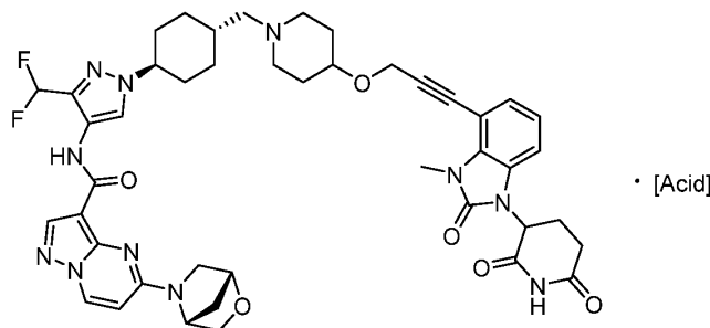
Formula A
