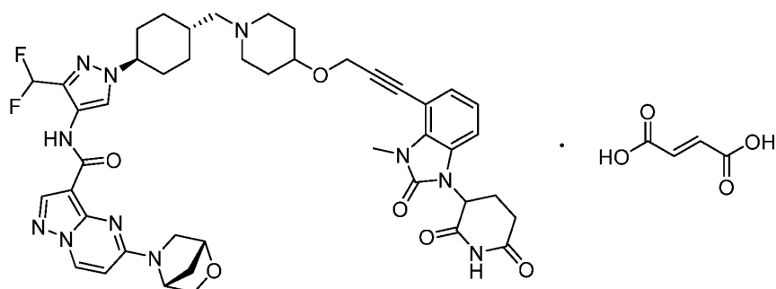
Compound 3
