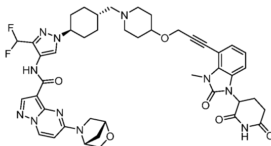
Compound 1
