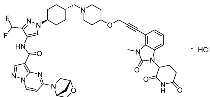
Compound 2
