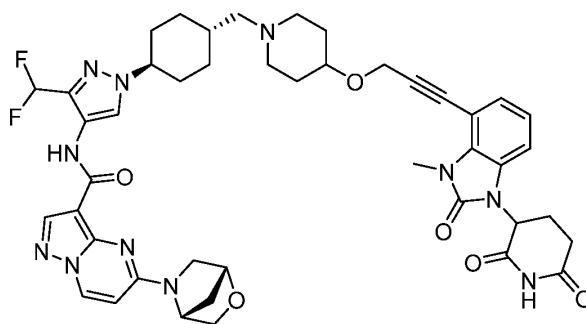
Compound 1
