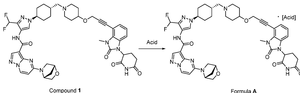
Scheme 2. Preparation of Salts of Formula A
