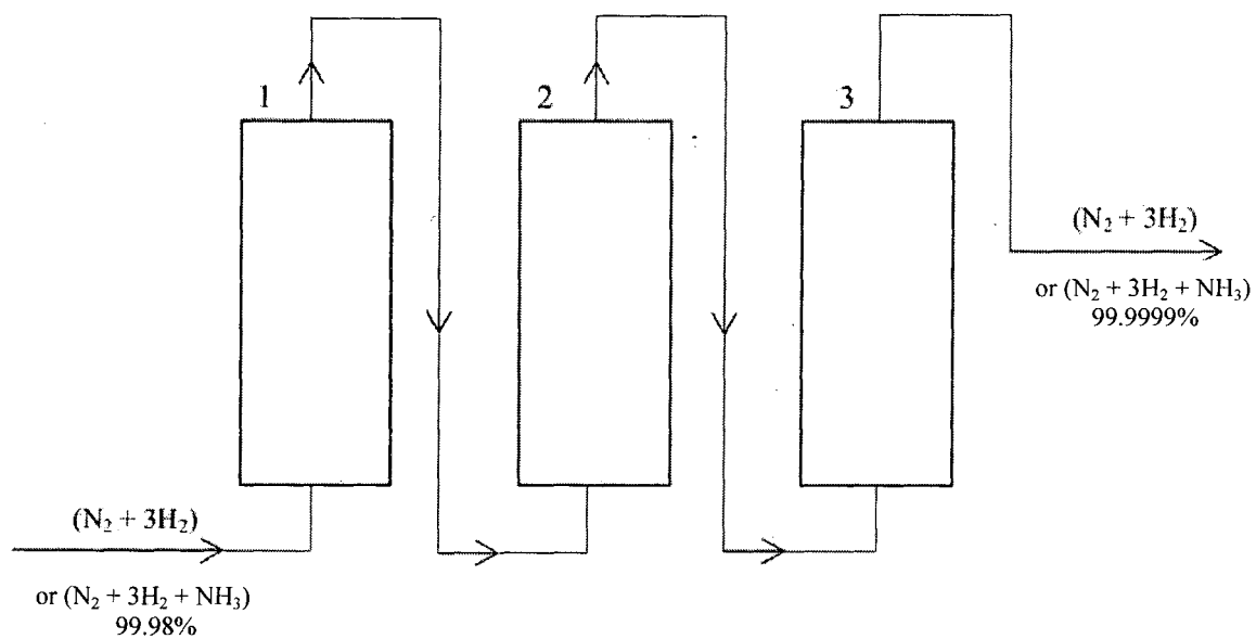
Fig. 2. Block diagram of the system according to Examples 2 and 3.
