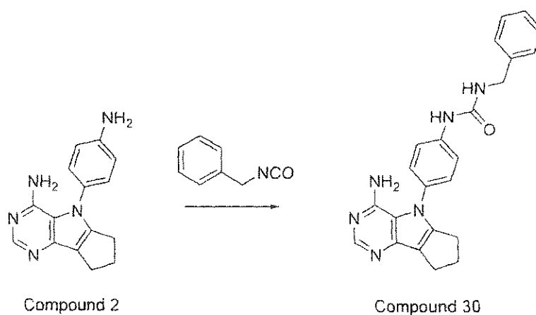
Scheme 7
