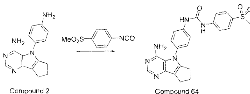
Scheme 19
