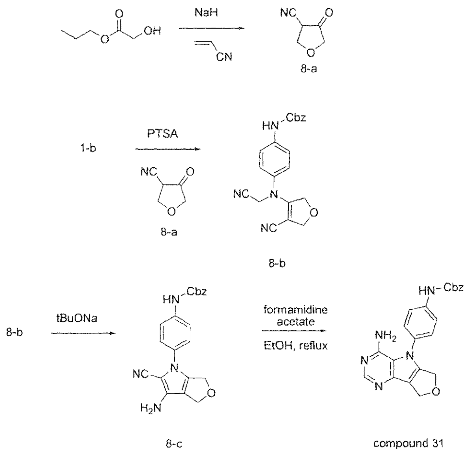
Scheme 8
