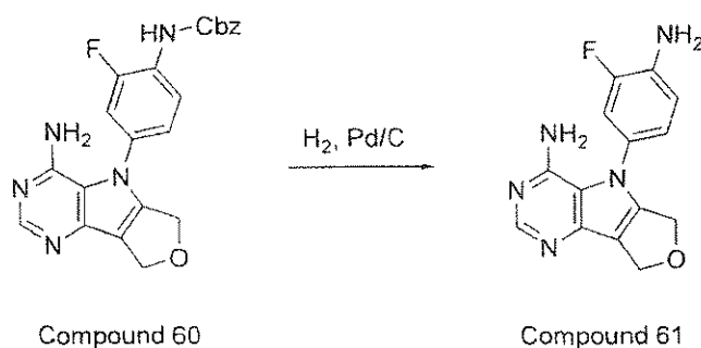
Scheme 16
