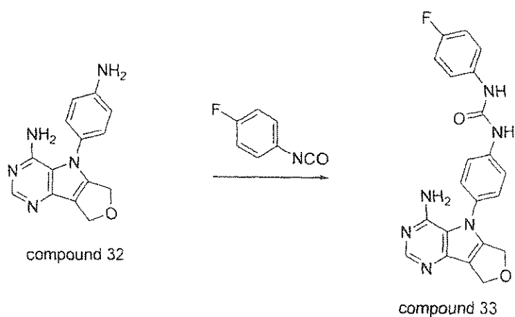
Scheme 10
