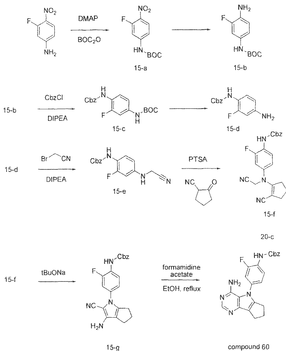
Scheme 15
