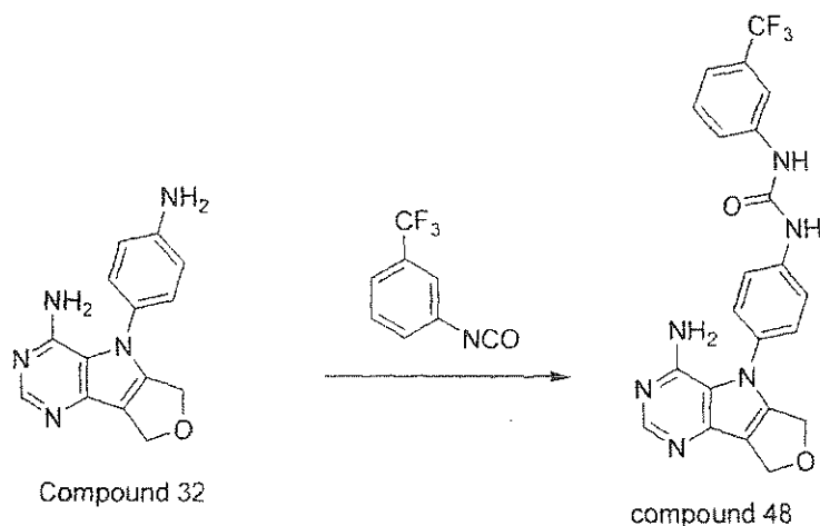
Scheme 14
