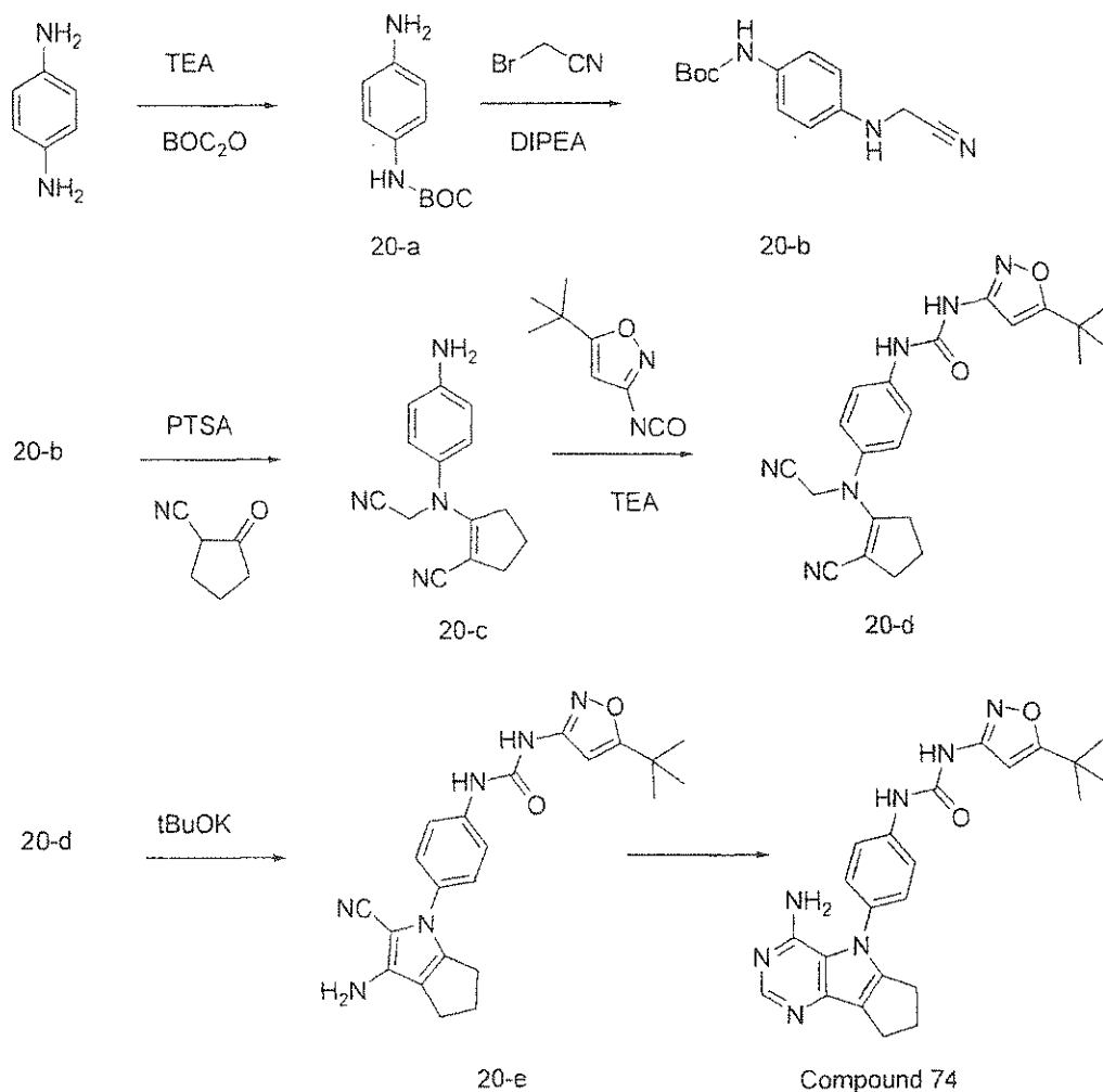
Scheme 20
