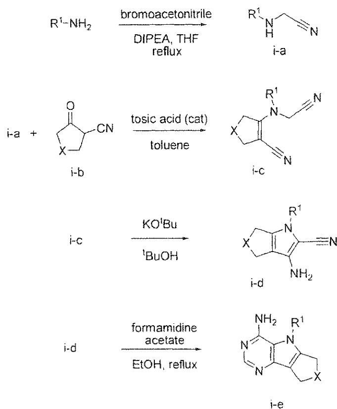
Scheme i
