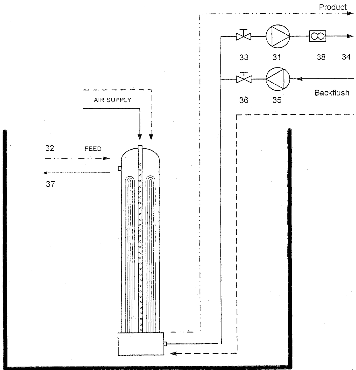
SUBMERGED CONFIGURATION
