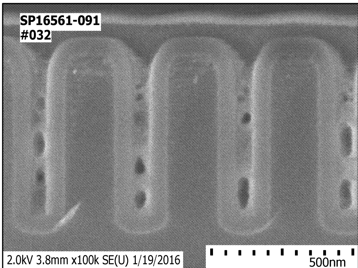
FIG. 1 (Prior Art)
