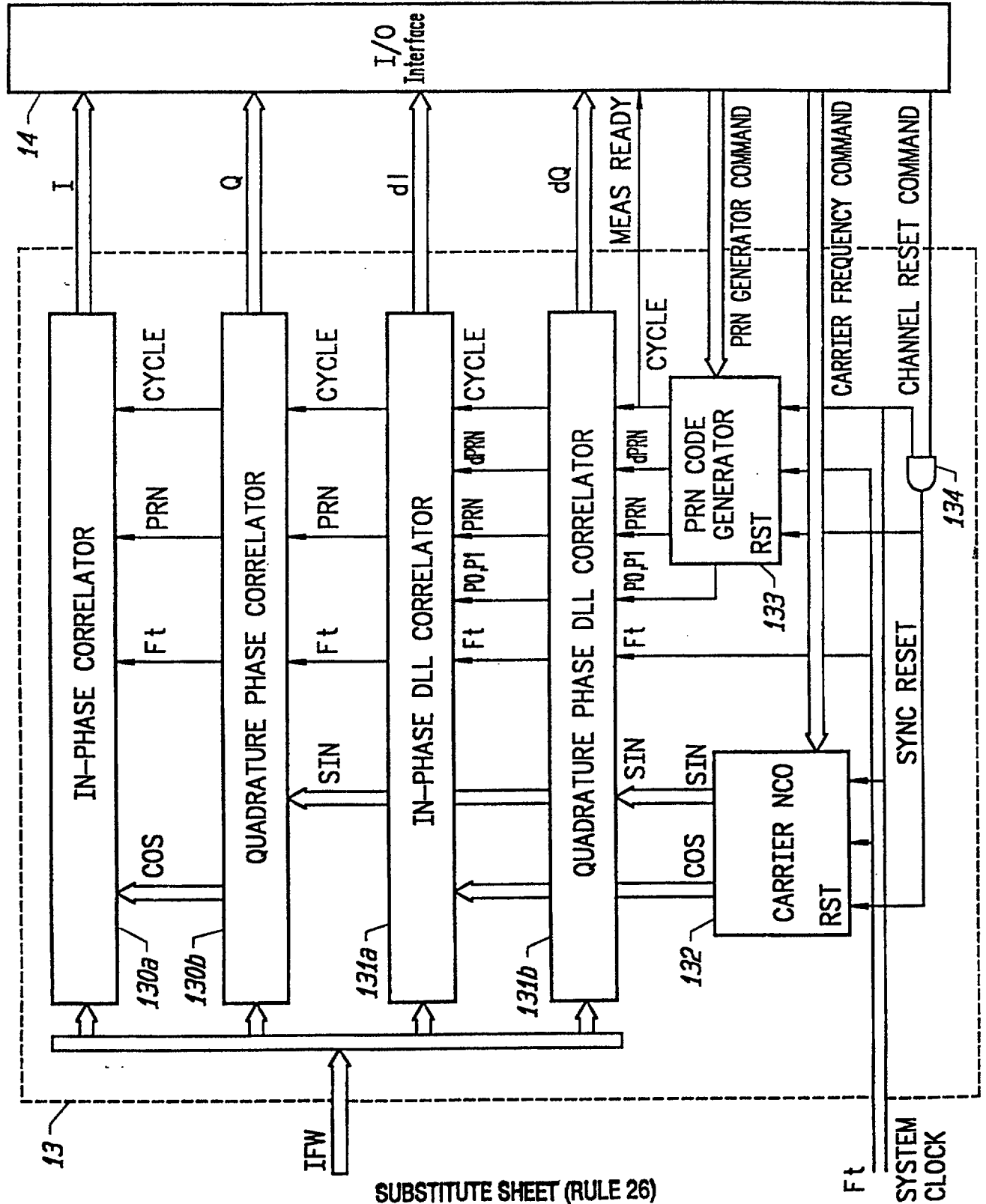
FIG. 16 (One Channel)
