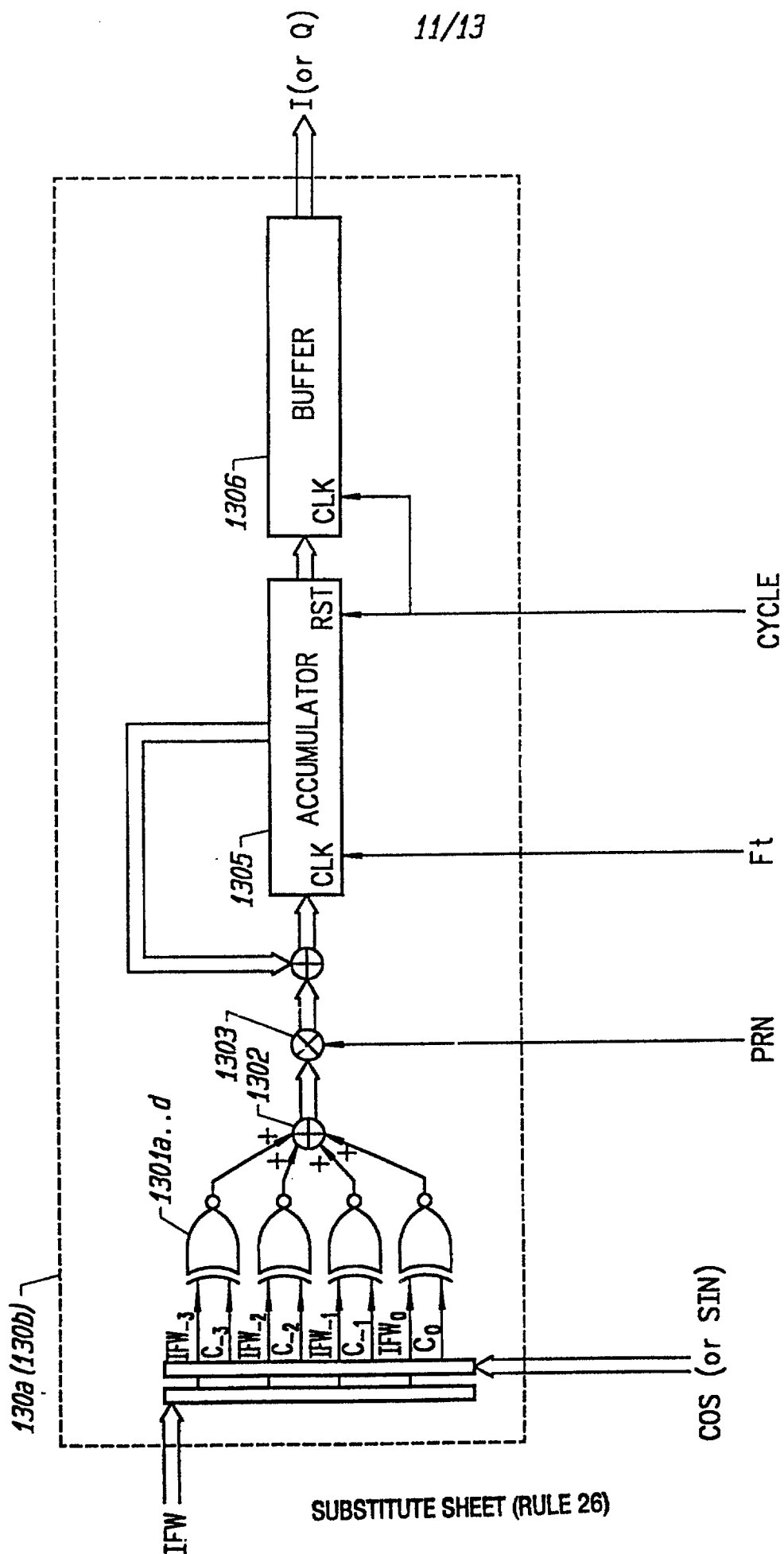
FIG. 19 (Correlator)
