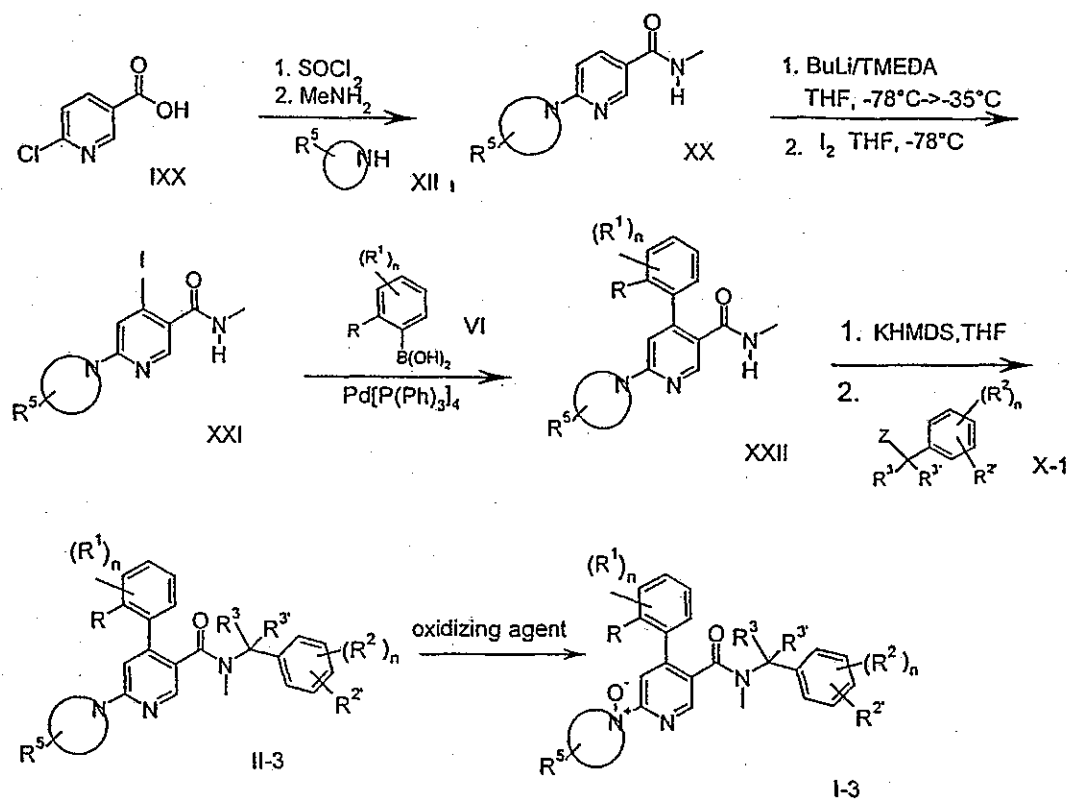
Scheme 3
