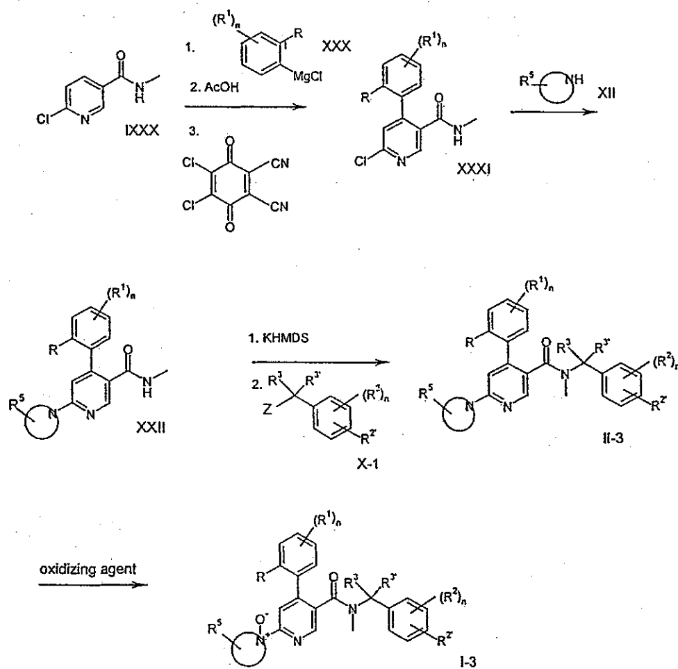
Scheme 6
