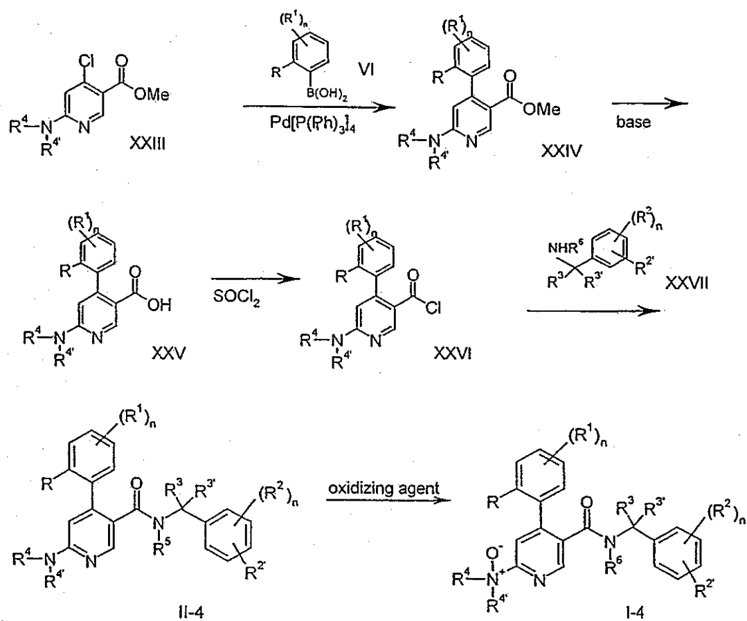
Scheme 4
