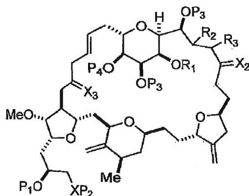
(IIIB);
