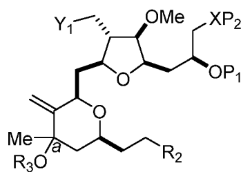
(VIIC),
