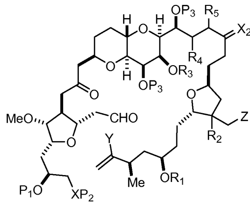
(VIA),
