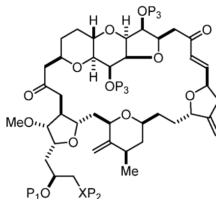
(IC),
