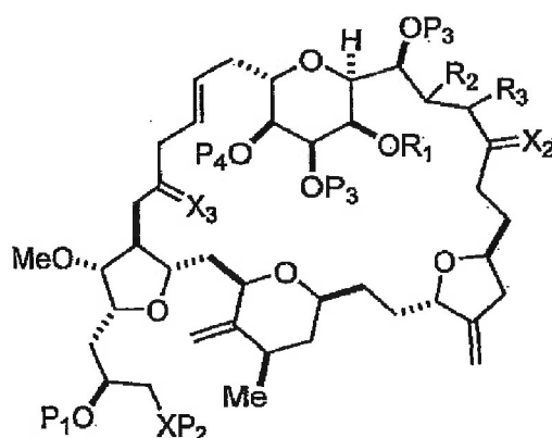
(IIIB);
