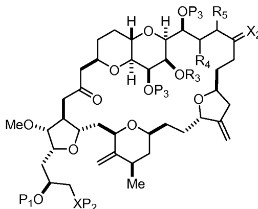
(VIC)
