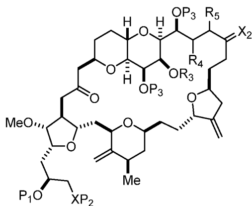
(VIC);
