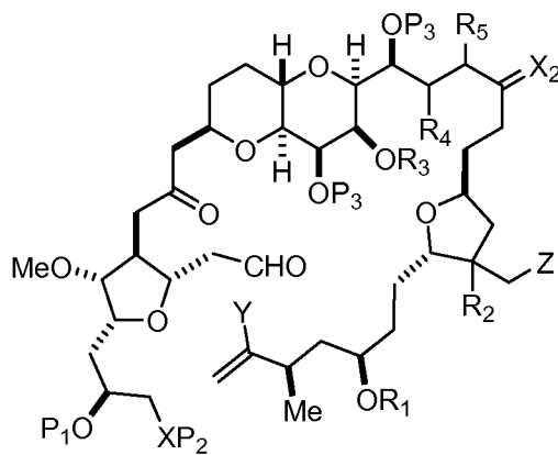
(VIA),
